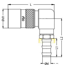
Socket / Kupplung
