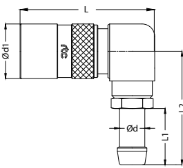
Socket / Kupplung
