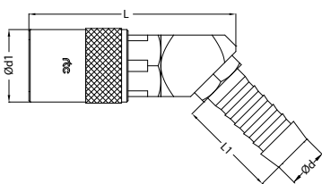
Socket / Kupplung
