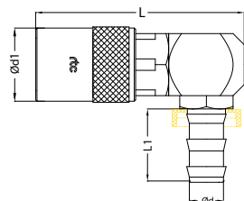
Socket / Kupplung
