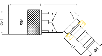
Socket / Kupplung
