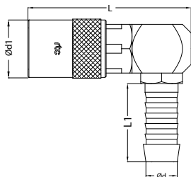
Socket / Kupplung
