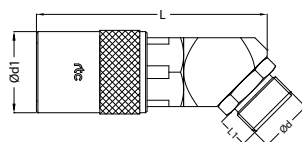
Socket / Kupplung
