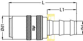
Socket / Kupplung
