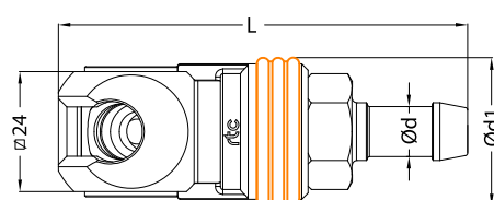
Socket / Kupplung
