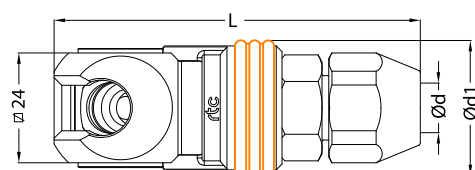
Socket / Kupplung
