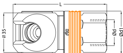
Socket / Kupplung
