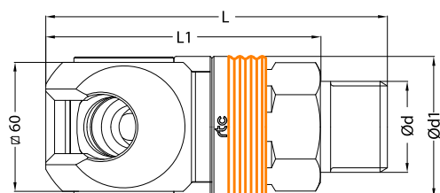
Socket / Kupplung
