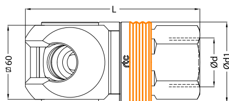
Socket / Kupplung
