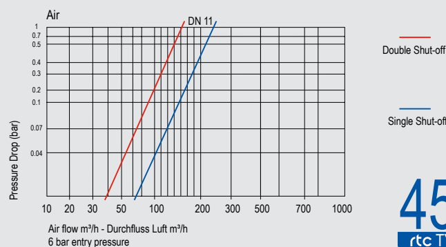
Flow Rate vs Pressure Drop Graph
