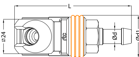
Socket / Kupplung
