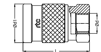
Free-Flow Coupling Kupplung ohne Ventil
